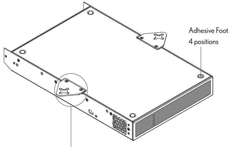
Diagram 4a THEORY DLC with desk/wall Mounting Plate and adhesive feet. 2 positions and 4 positions.
